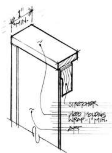
Wood Wrapped Stretcher (1" min.)
